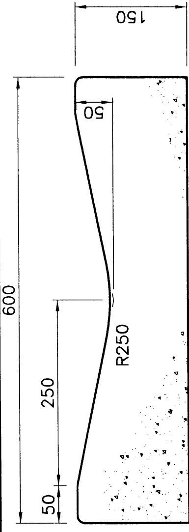
DISH DRAIN
