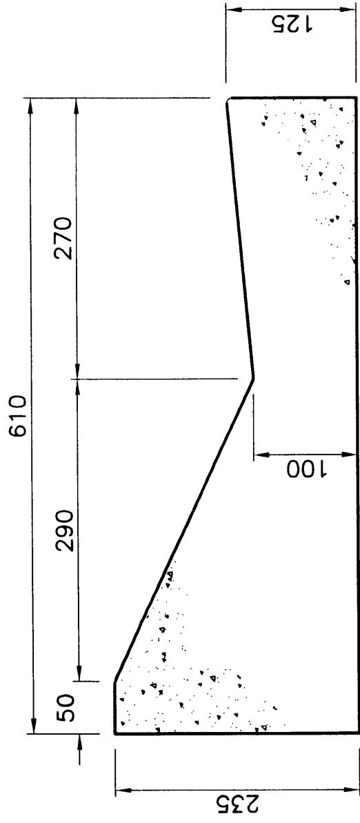
MOUNTABLE KERB AND CHANNEL
