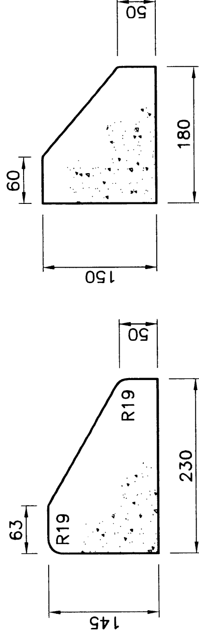
MEDIAN KERB
